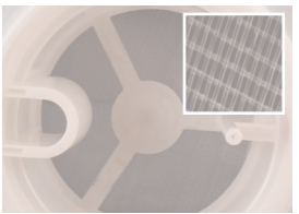
Tank filter port diameter: 0.5mm (max)
